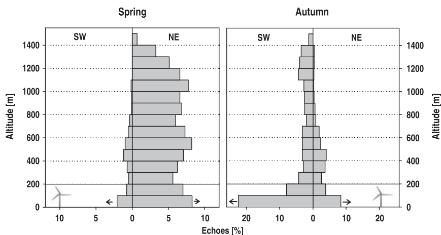
Figure 6. Nocturnal migration directions as recorded by vertical radar at research platform FINO 1 in different altitudes in spring 2004 (left, n = 2128 echoes) and in autumn 2003 and 2004 (right, n = 3159 echoes). Only tracks with a length of at least 35 m were used. Echoes of low flying birds cannot be separated from reflections of the sea surface. Thus, the arrows emphasize that the proportion of echoes in the stratum from 0 to 100 m is presumably greater. The line at 200 m represents the approximate maximum height of the future offshore wind energy plants. Note different scaling of x-axes.
