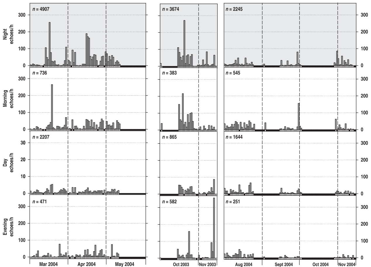
Figure 4. Migration intensity (number of corrected echoes per hour and day, n = number of uncorrected echoes) of single observation days in spring (2004, left) and autumn (2003 and 2004, right) in four different periods of the day (for definitions see Methods) at research platform FINO 1. Black bars under histograms indicate periods without radar measurements.
