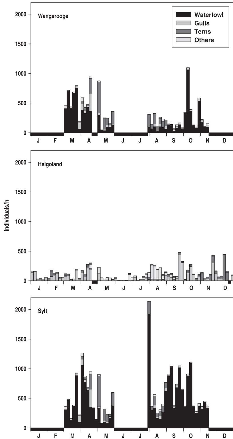
Figure 2. Mean migration intensity per 5-day period (pentade) recorded by sea-watching on the islands of Wangerooge ( n = 85\,538 ), Helgoland ( n = 87\,098 ) and Sylt ( n = 238\,765 ) for main species groups (July 2003 to December 2004). Black bars under histograms indicate periods without sea-watching.
