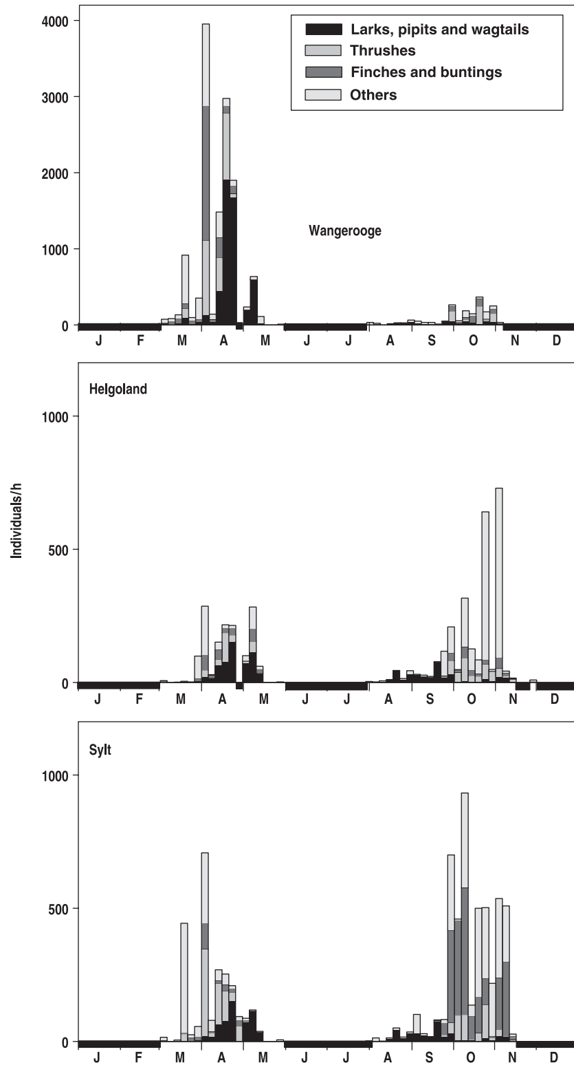
Figure 3. Mean migration intensity per 5-day period (pentade) recorded by passerine passage counts on the islands of Wangerooe ( n = 70\ 302 ), Helgoland ( n = 21\ 908 ) and Sylt ( n = 67\ 670 ) for main species groups (August 2003 to November 2004). Black bars under histograms indicate periods without counts. Note variable scaling of the y-axes.
