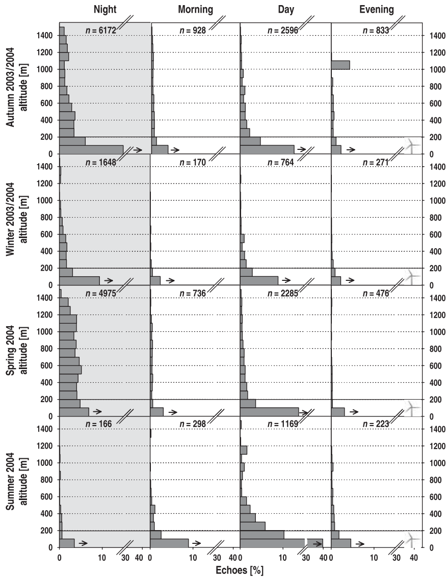
Figure 5. Flight altitudes (percentage of corrected echoes per altitude stratum, n = number of uncorrected echoes) in different seasons and times of day (for definitions see Methods) at research platform FINO 1. Seasonal totals = 100%. Echoes of low flying birds cannot be separated from reflections of the sea surface. Thus, the arrows emphasize that the proportion of echoes in the stratum from 0 to 100 m is presumably greater. The line at 200 m represents the approximate maximum height of the future offshore wind energy plants.
