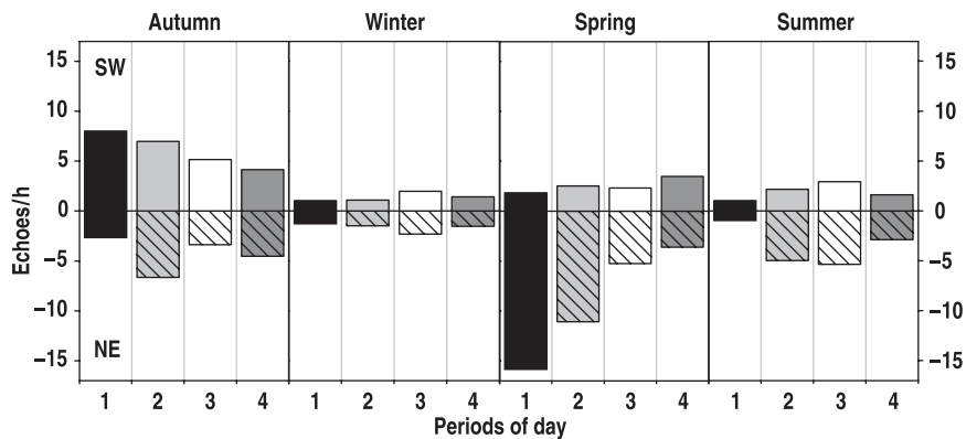
Figure 7. Nocturnal migration directions as recorded by vertical radar at research platform FINO 1 in different seasons and periods of day in autumn 2003 and 2004, in winter 2003/04, in spring 2004 and in summer 2004. Only tracks with a length of at least 35 m were used. 1 = night, 2 = morning, 3 = day, 4 = evening (for definitions see Methods). Positive values = crude direction southwest, negative values = crude direction northeast.
